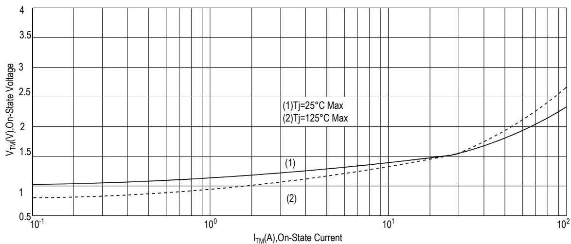
FIG.5: On-state characteristics(Max)
