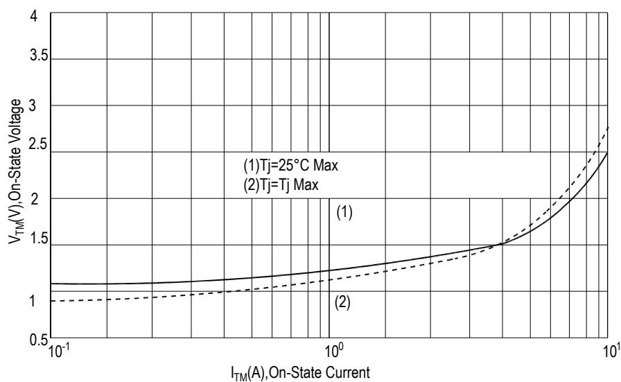
FIG.5: On-state characteristics(Max)
