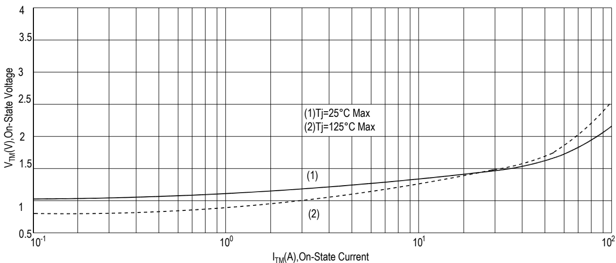
FIG.5: On-state characteristics(Max)
