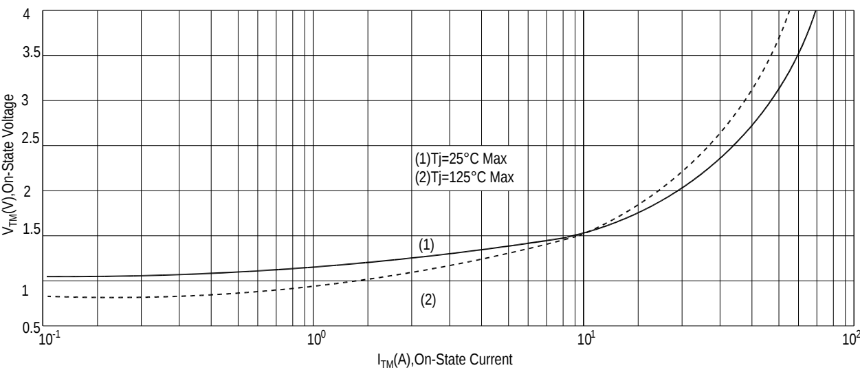
FIG.9: On-state characteristics(Max)
