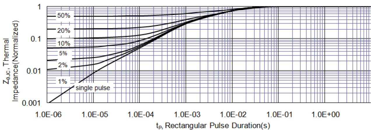
Figure 11: Maximum Effective Thermal Impedance, Junction-to-Case
