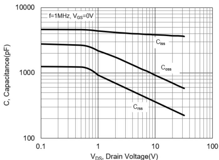
Figure 5: Capacitance Characteristics
