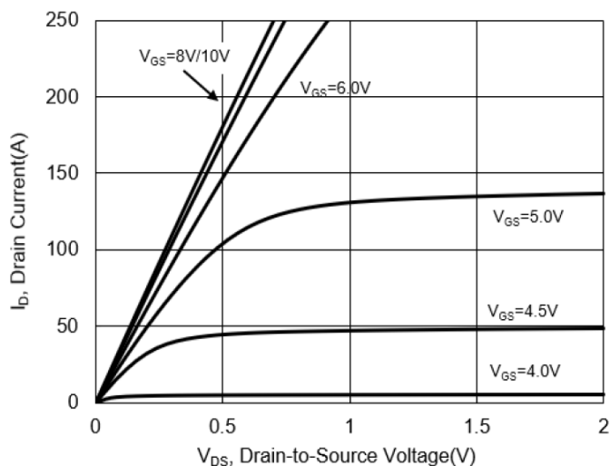
Figure 3: Drain Current
