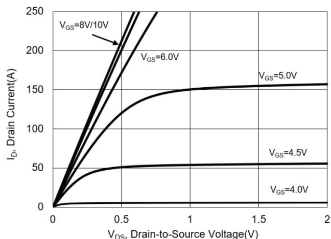
Figure 3: Drain Current
