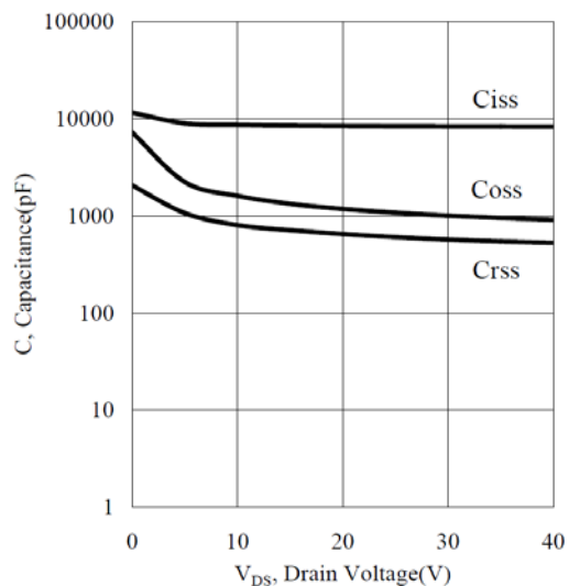
Figure 5: Capacitance Characteristics
