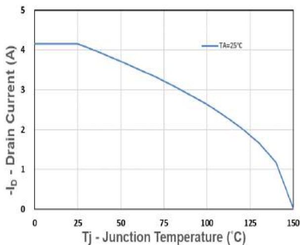
Figure 5: Drain Current.
