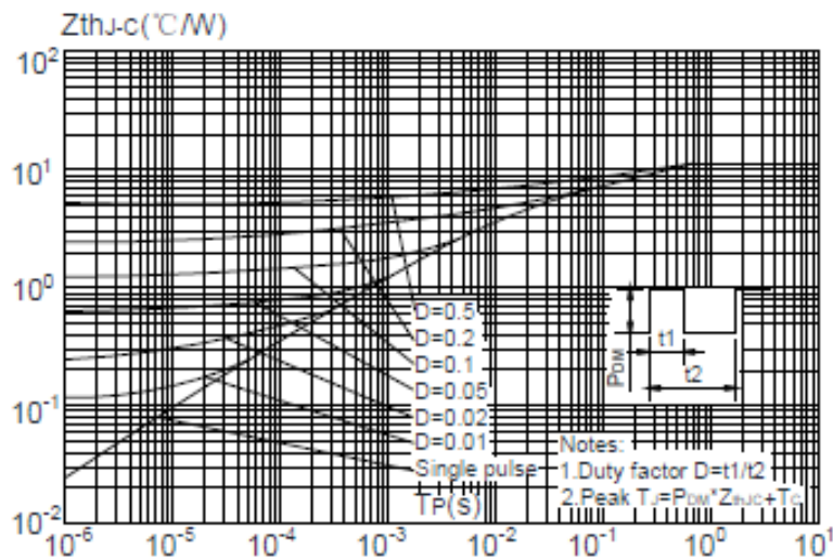
Figure 9: Effective Transient Thermal Impedance
