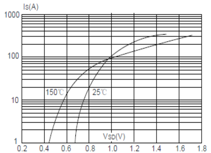
Figure 8: Typical Source-Drain Diode Forward Voltage
