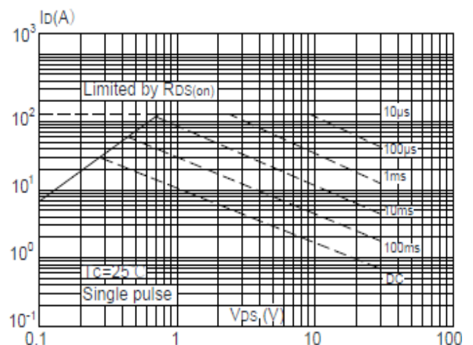
Figure 6: Maximum Safe Operation Area
